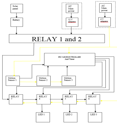
Figure 2.1 General Diagram of the System.
