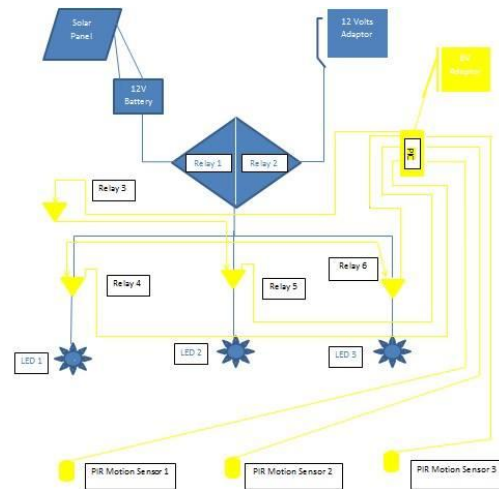
Figure 3.2Block Diagram of the Lighting System.
