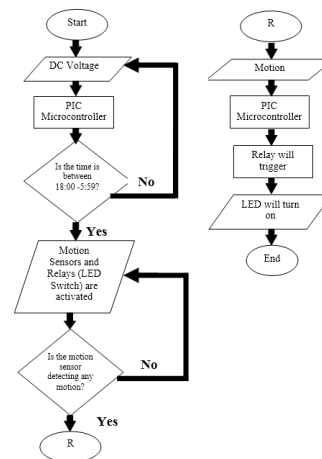
Figure 2.3 Flow Chart of the automated Lighting System
